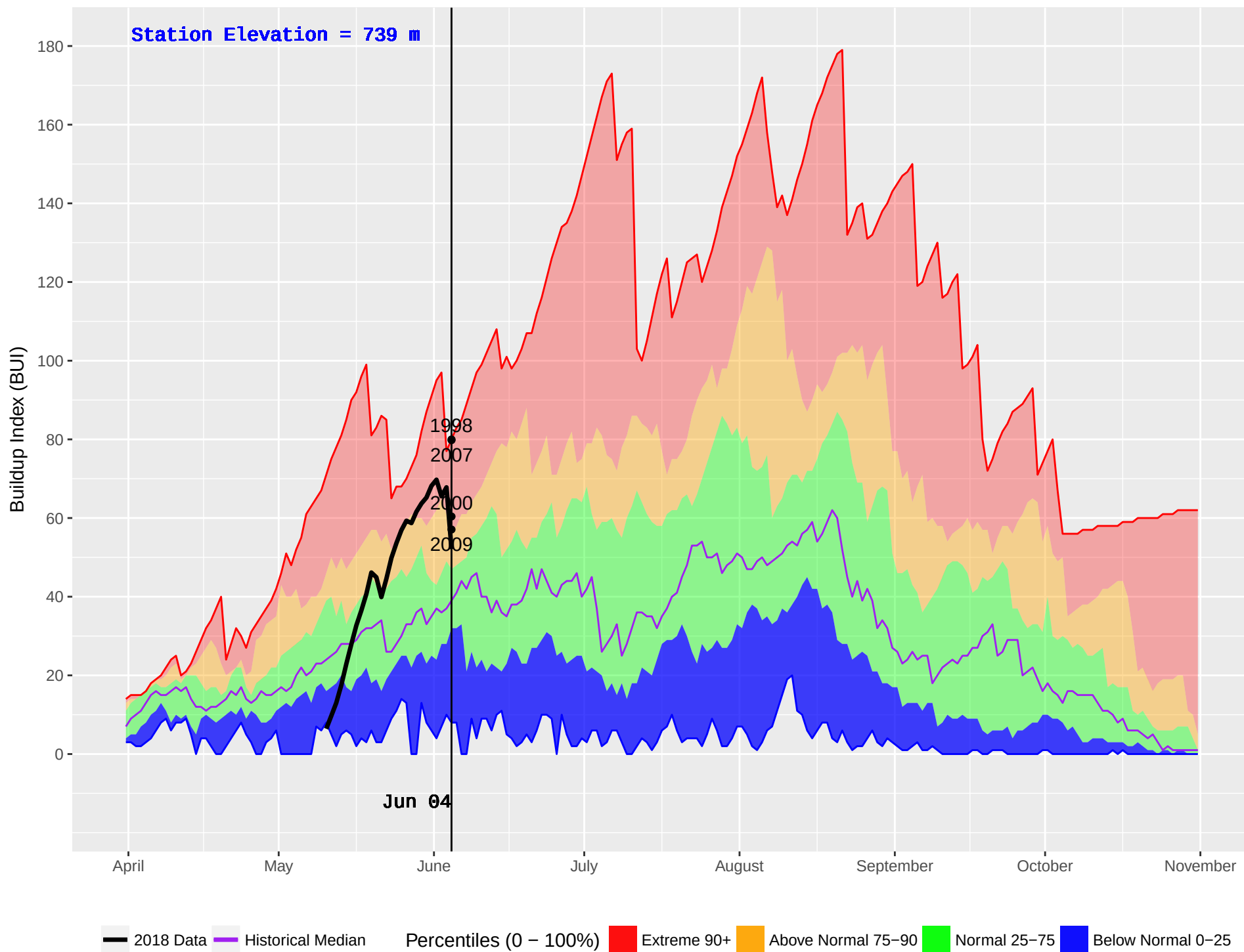
BEAR LAKE (149) : Historical (1980–2016) and Current (2018) Noon Buildup Index (BUI)
